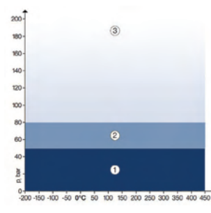
pT diagram for thickness 2.0 mm
