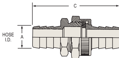
Short Shank Garden Hose Fitting Set 1 (Hex Nut)
