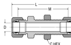
Bulkhead Union 62CBH
