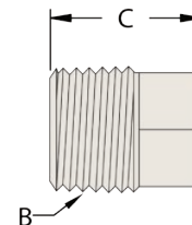
Square Head Plug-Solid PTFE-SAE Short-Lead-Free C270/ANSI 372 Ref SAE J531
