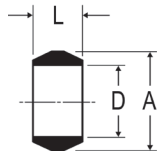
Sleeve 60C Reference SAE 060115
