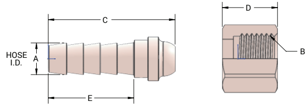
Welding Hose Coupling Right Hand Thread for Oxygen Line
