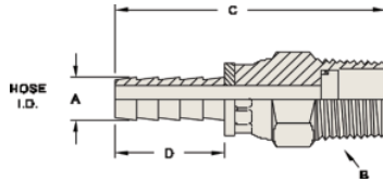
NPTF-Male Swivel Hose Barb National Pipe Tapered-Dryseal
