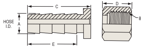
NPSM-Female Swivel Hose Barb National Pipe Straight-Gasket Seat Type
