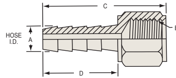
NPTF-Female Hose Barb-Solid National Pipe Tapered-Dryseal
