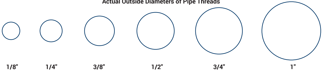
Actual Outside Diameters of Tubing
