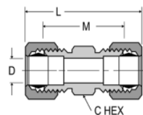
Union 62C Reference SAE 060101 BA
