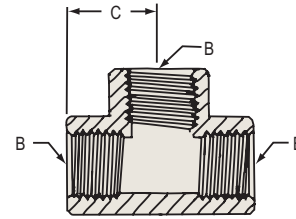
Female Pipe Tee-Extruded NPTF-Dryseal Ref. SAE 130438
